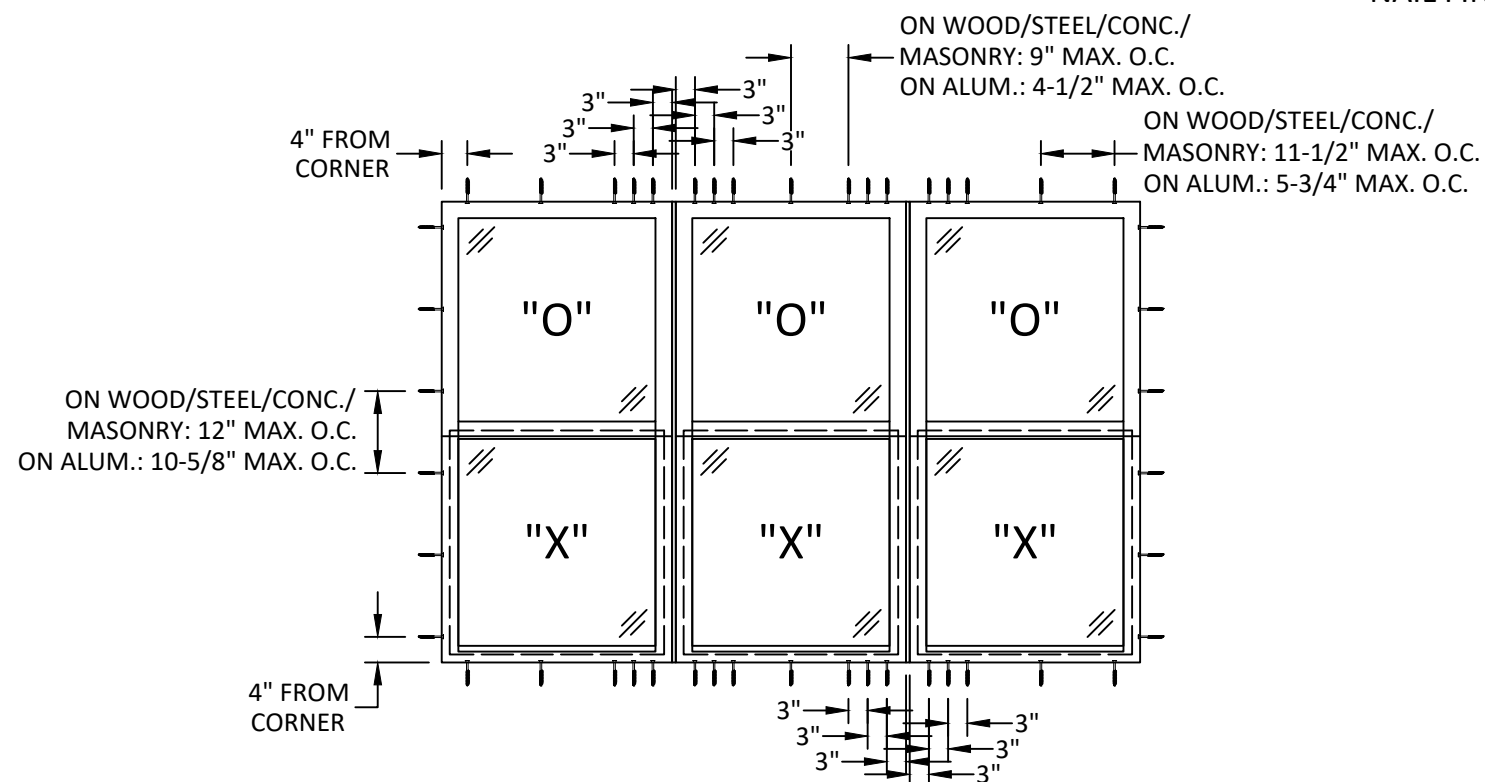
ANCHOR LAYOUT THROUGH FRAME
