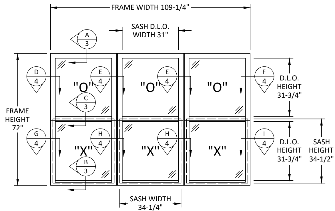
TYPICAL ELEVATION
