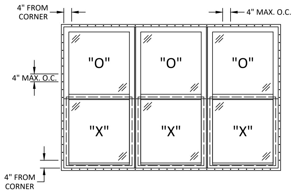
ANCHOR LAYOUT NAIL FIN
